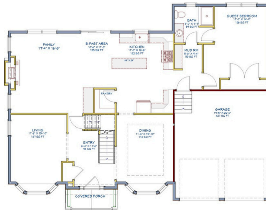
First Floor
