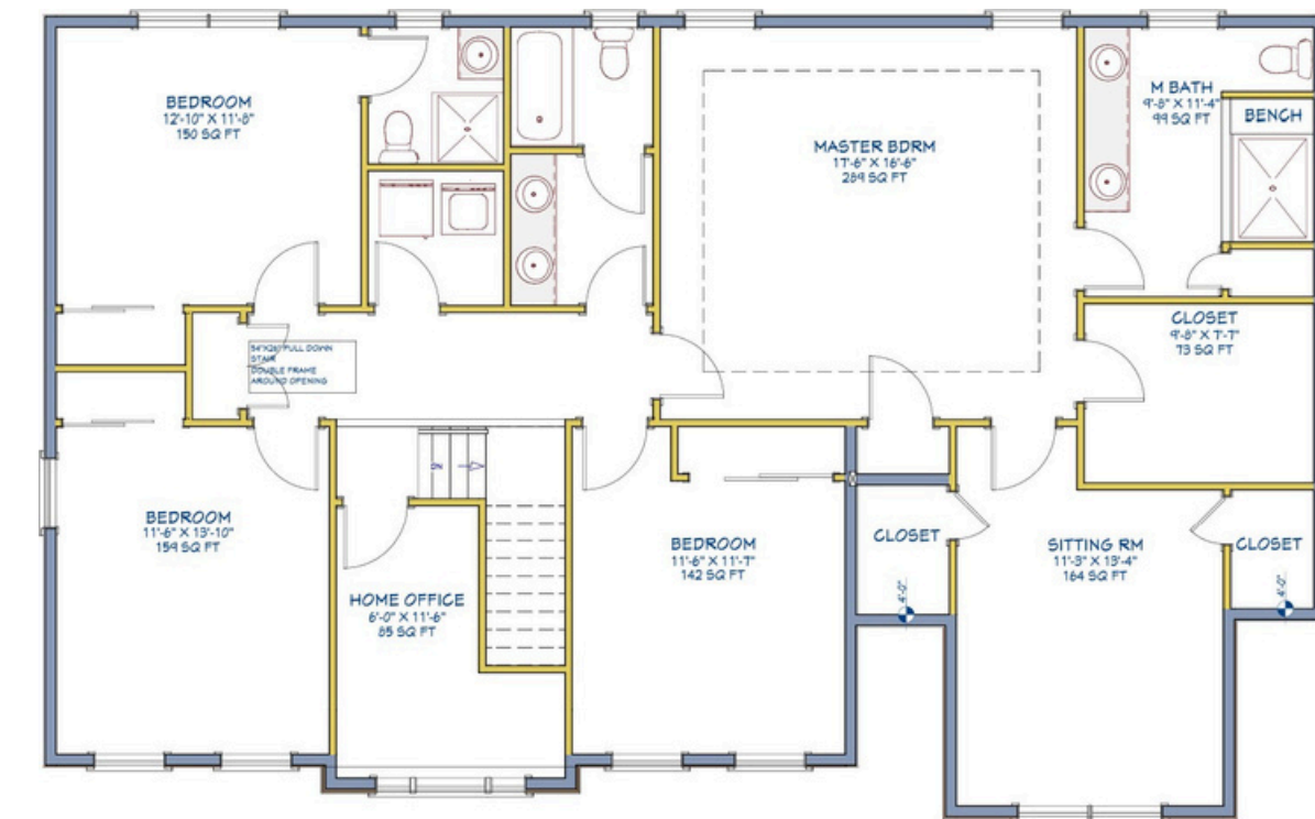
Second Floor
